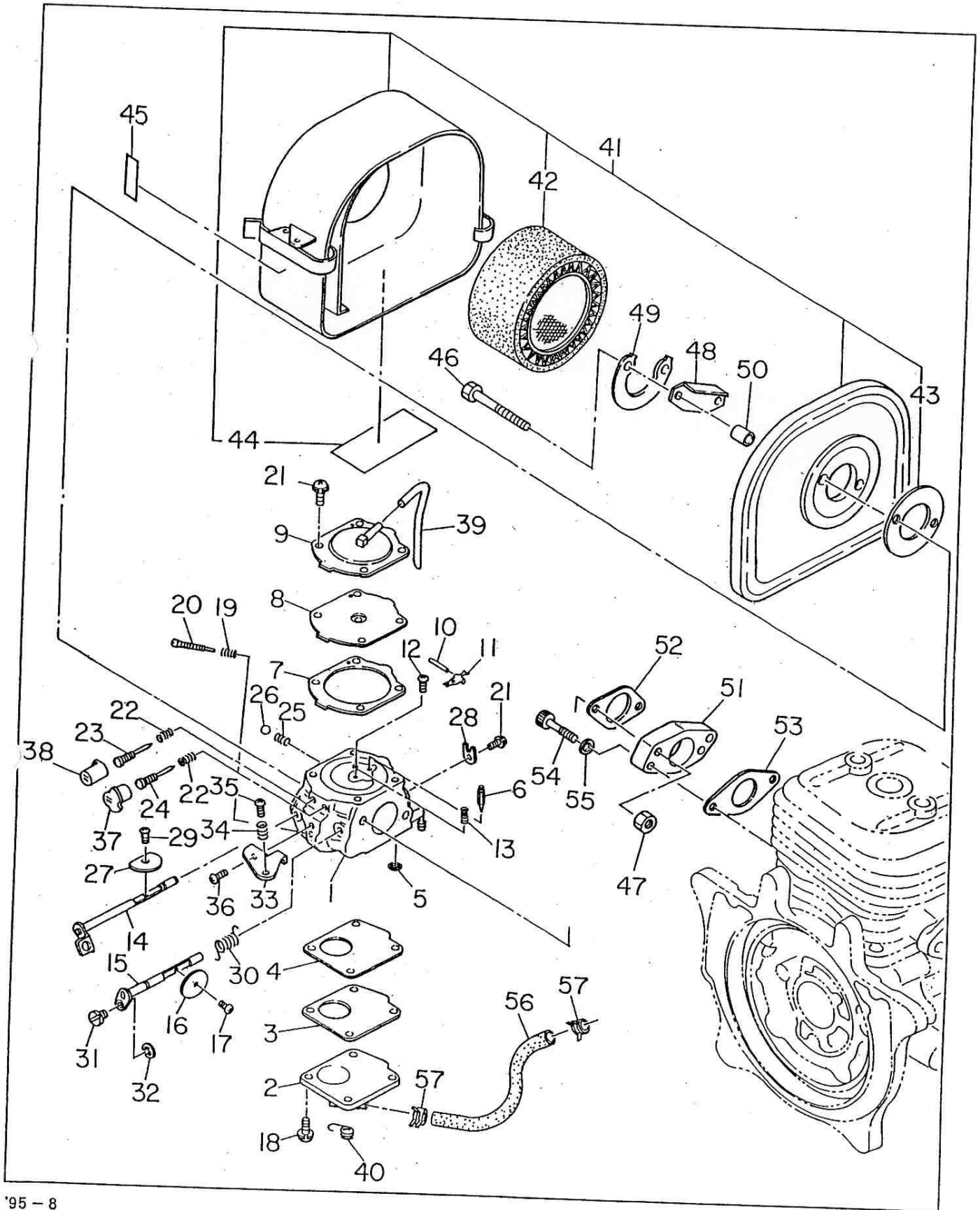
FIG. 5 CARBURETOR and AIR CLEANER
