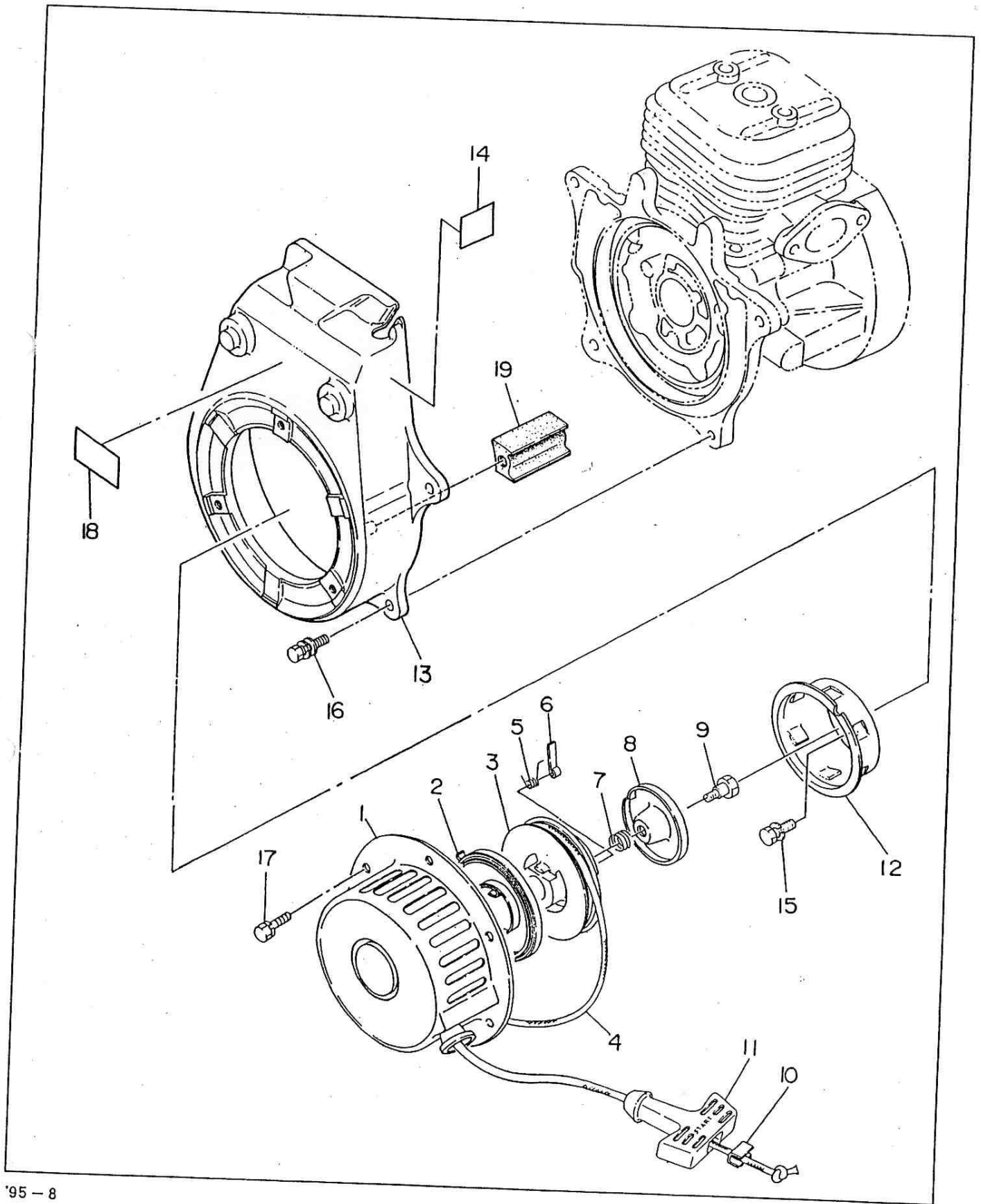
FIG. 4 RECOIL STARTER and BLOWER HOUSING
