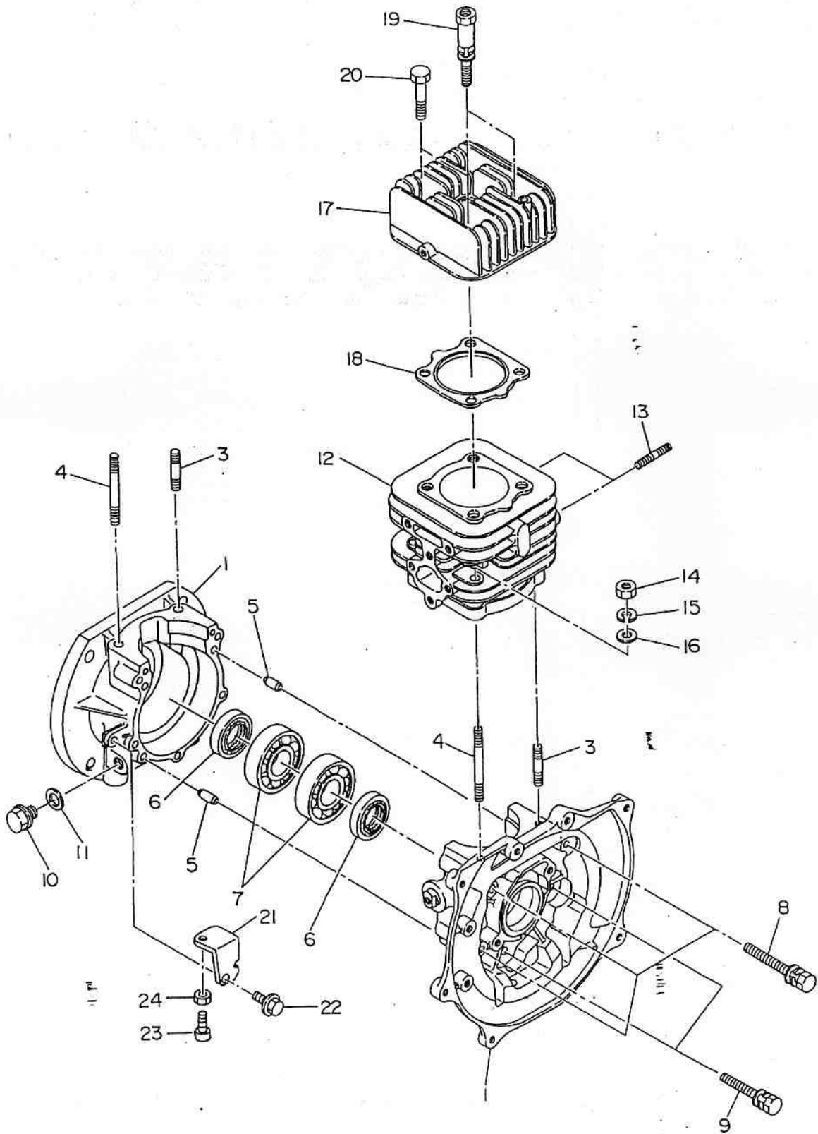
FIG. 1 CRANKCASE and CYLINDER HEAD
