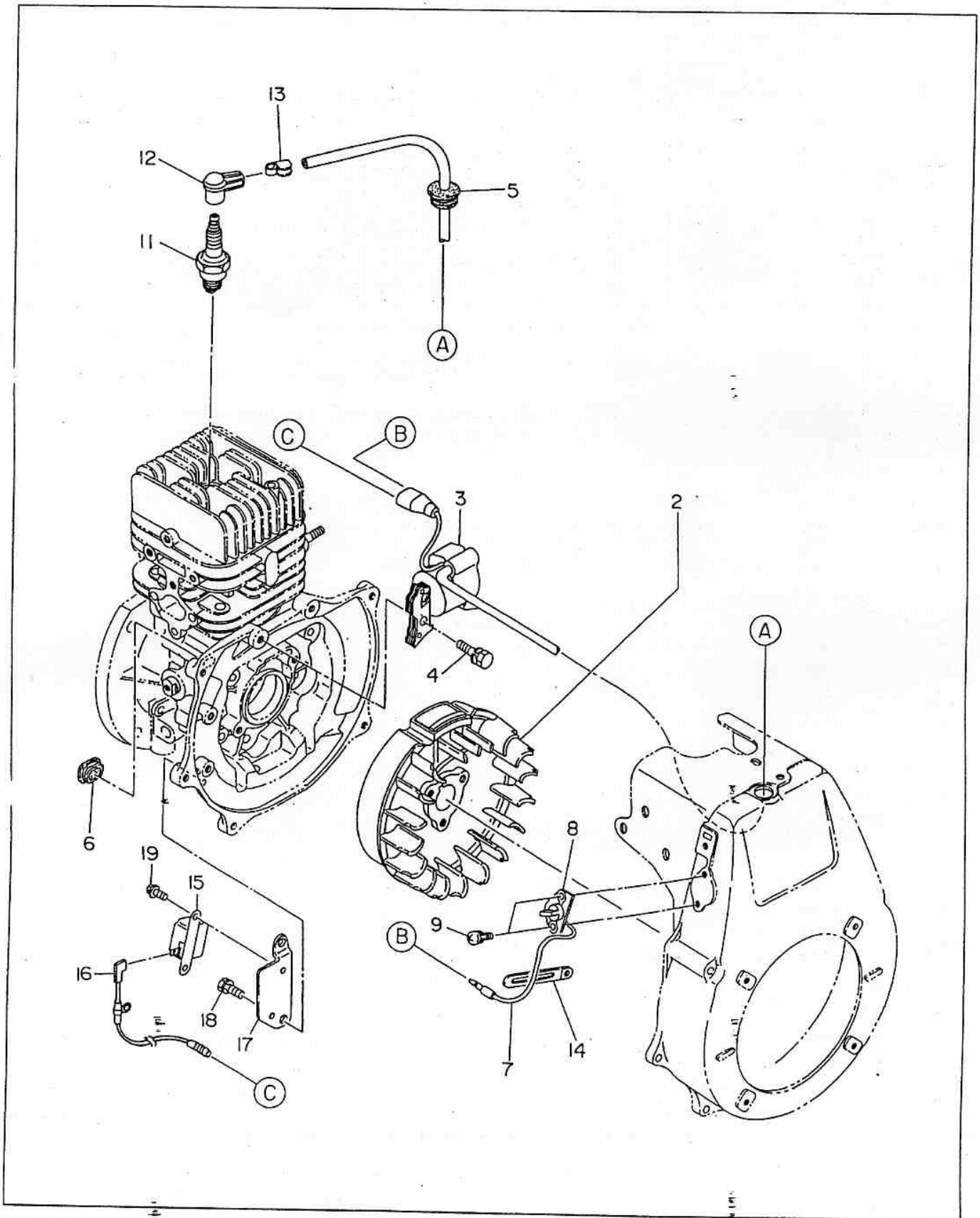
FIG. 5. ELECTRIC DEVICE
