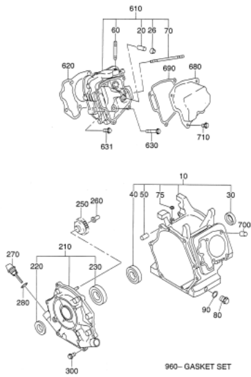
960-GASKET SET
